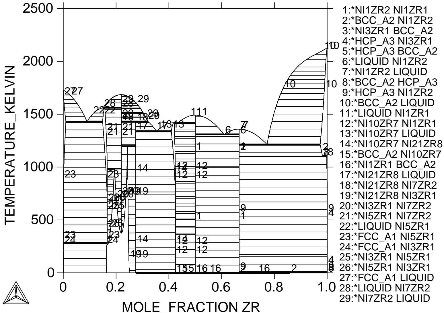
Calculated Ni-Zr phase diagram assessed by 1994Gho
