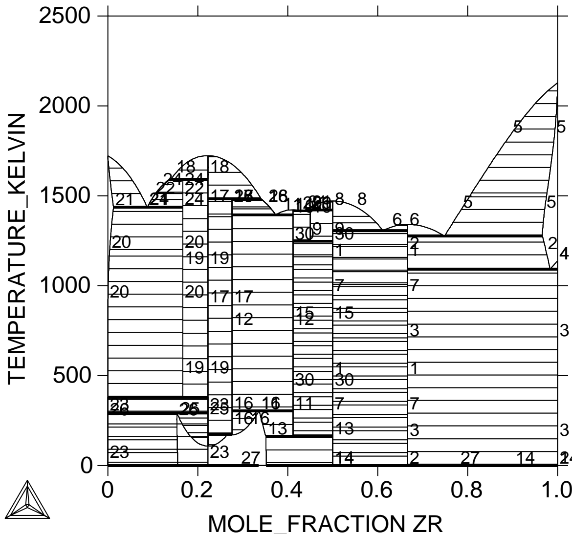
Calculated Ni-Zr phase diagram assessed by 2006Abe
