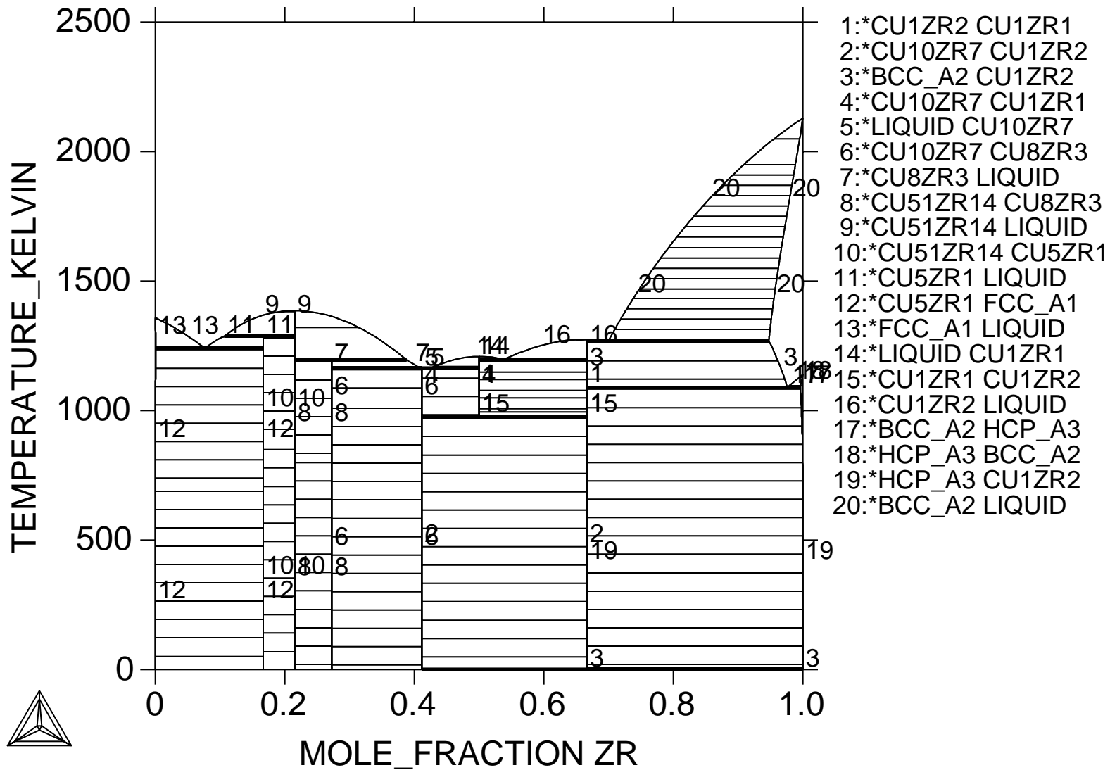
Calculated Cu-Zr phase diagram assessed by 1994Zen
