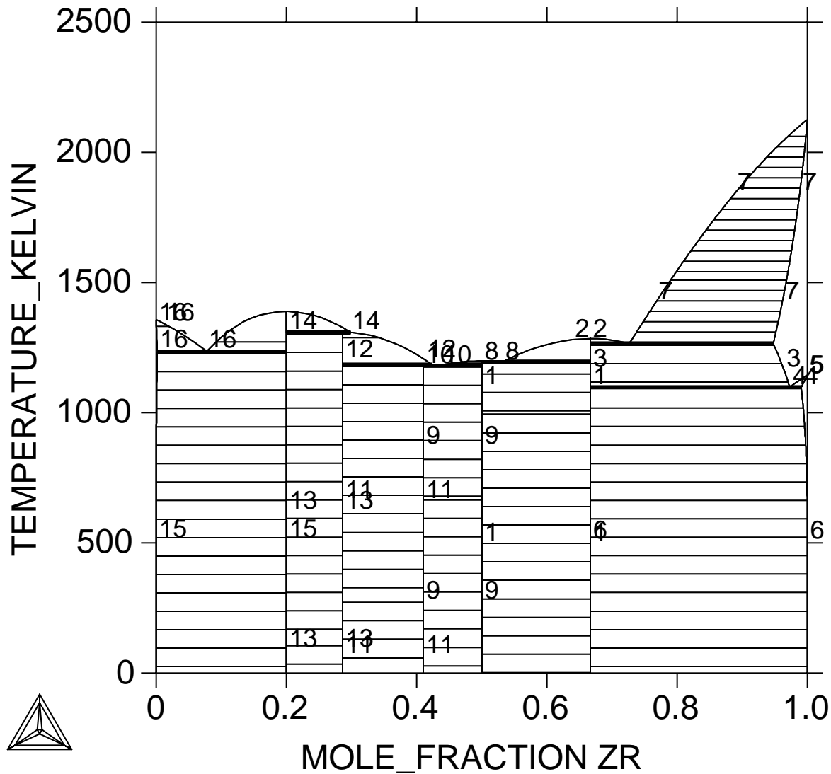
Calculated Cu-Zr phase diagram assessed by 1985Sau
