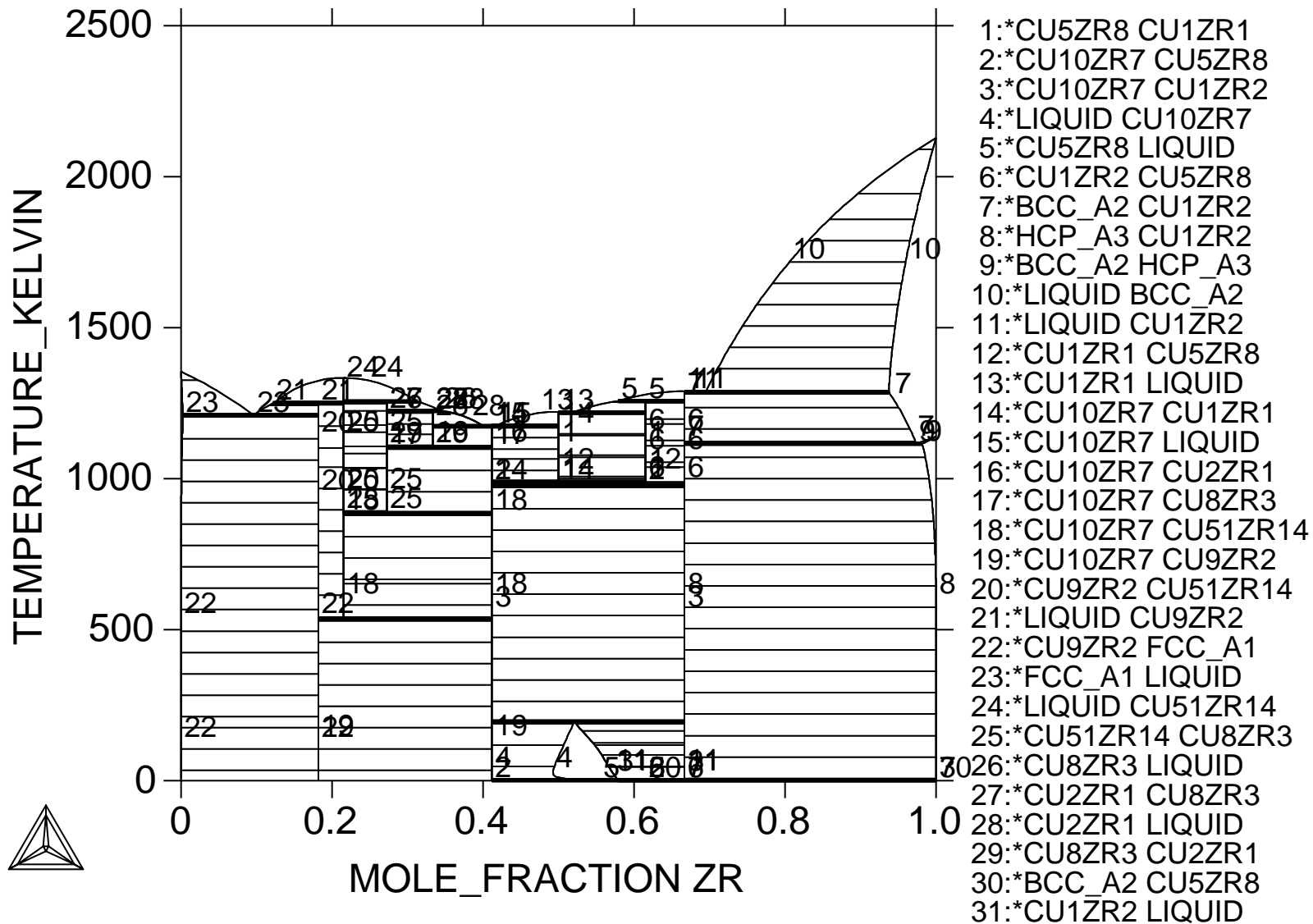
Calculated Cu-Zr phase diagram assessed by 2006Abe
