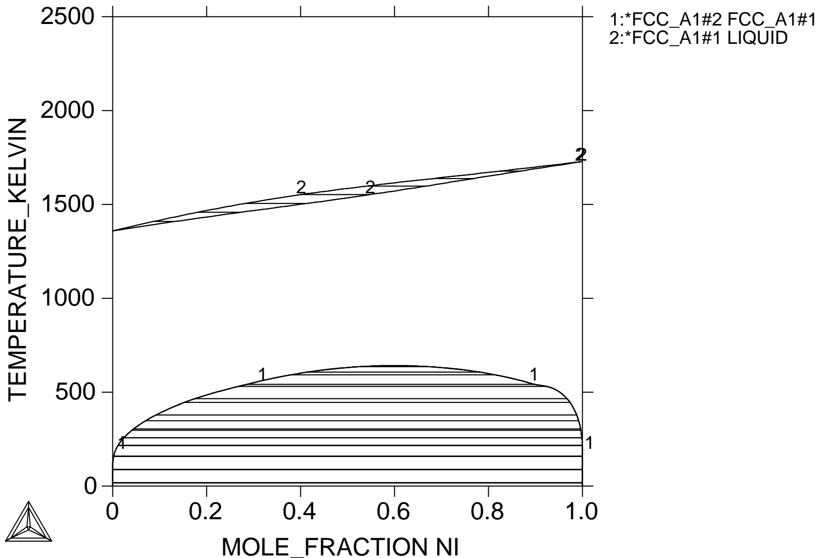
Calculated Cu-Ni phase diagram assessed by 1992Mey
